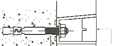
SECTION THRU A NTS
